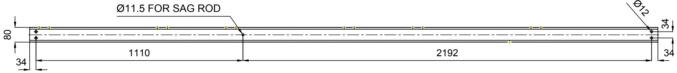
FRONT VIEW
