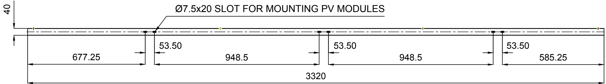
FRONT VIEW
