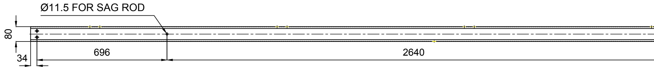
FRONT VIEW
