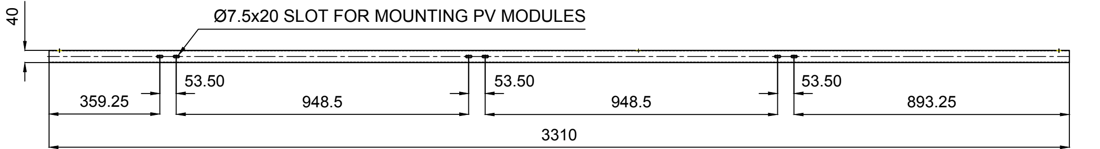
FRONT VIEW
