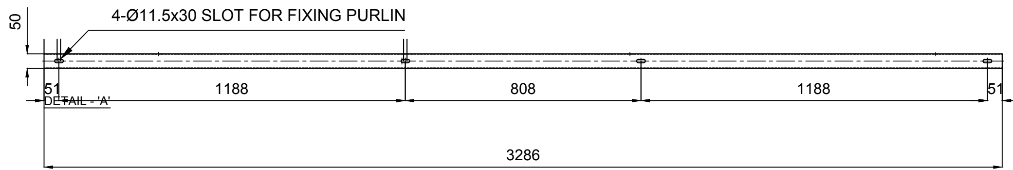
TOP VIEW
