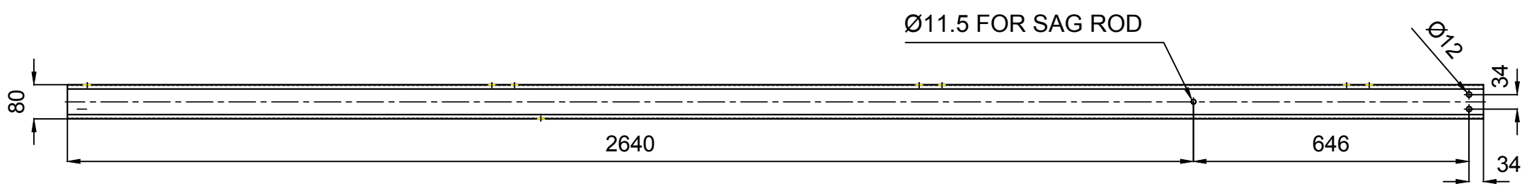
FRONT VIEW
