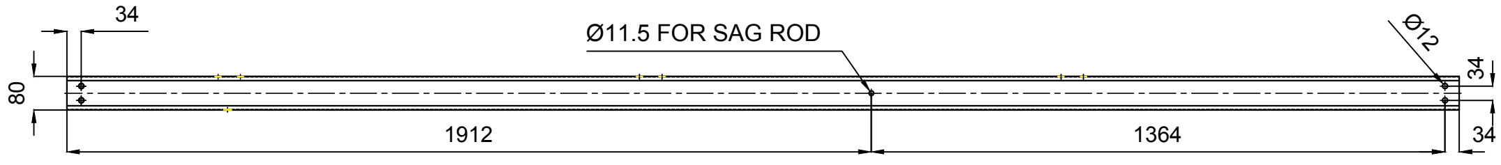
FRONT VIEW
