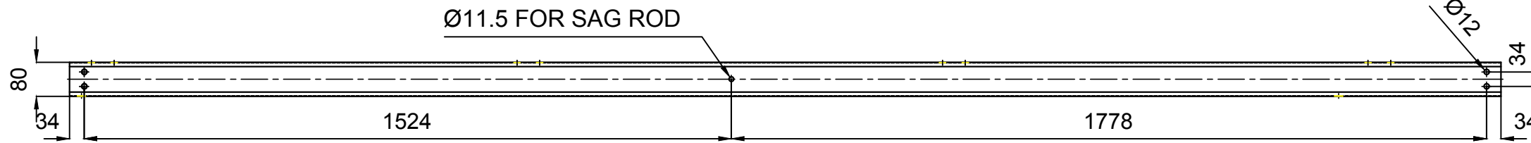
FRONT VIEW
