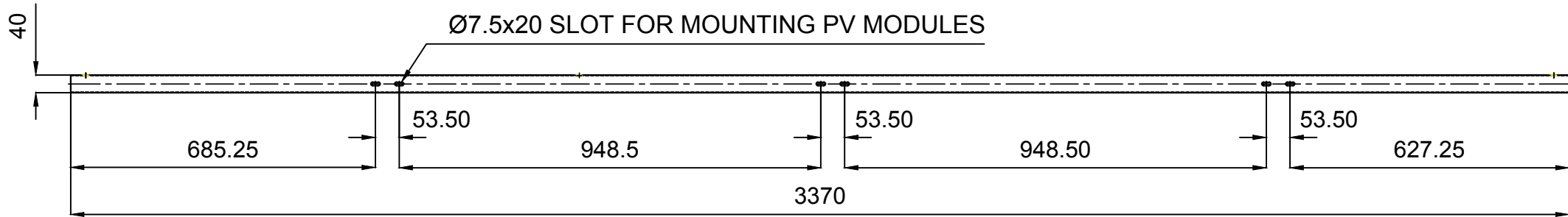
FRONT VIEW
