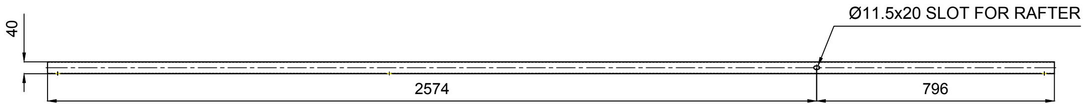
BOTTOM VIEW
