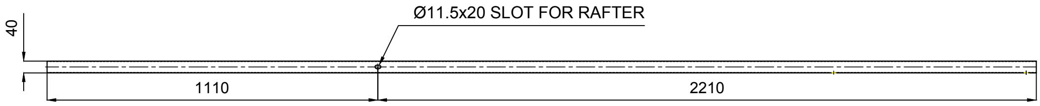
BOTTOM VIEW
