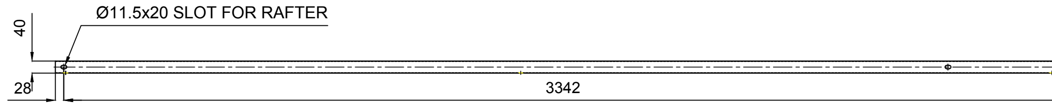
BOTTOM VIEW
