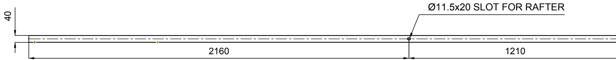
BOTTOM VIEW
