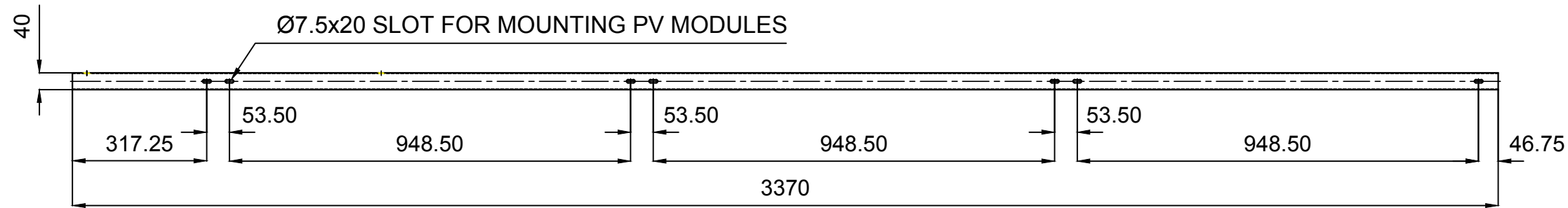
FRONT VIEW
